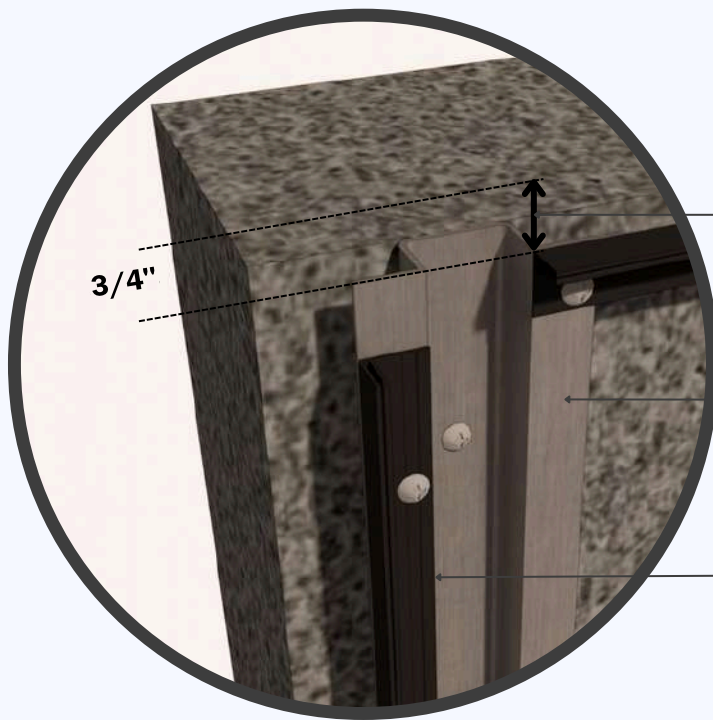
DETAIL PVC Base Siding 6" & 4" Quik-Trim System
