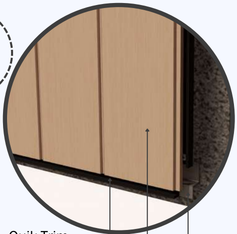
DETAIL Siding 6" & 4" Quik-Trim System
