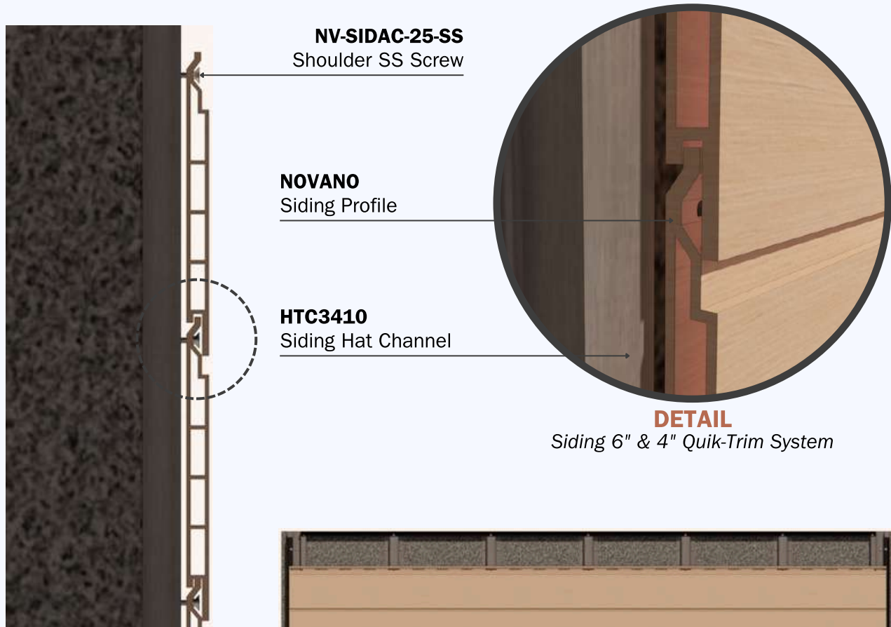
SECTION Siding 6" & 4" Quik-Trim System
