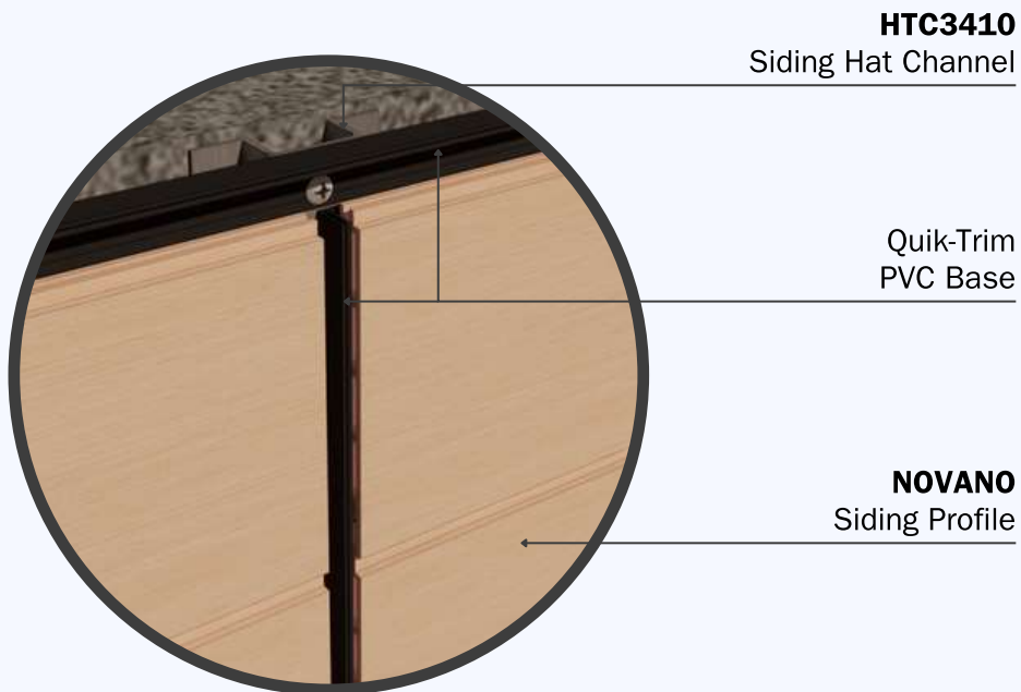
DETAIL Siding 6" & 4" Quik-Trim System
