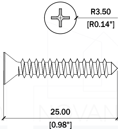
5 SCREW DETAILS D 6 SCALE 1:0.50 MTRS 25MM
