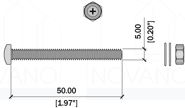
5 NUT & BOLT DETAILS
