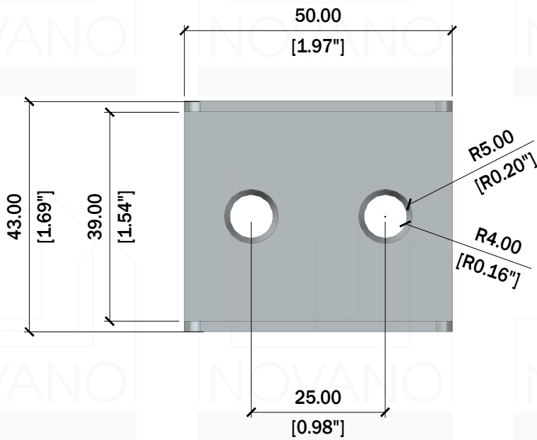
4 PLAN
